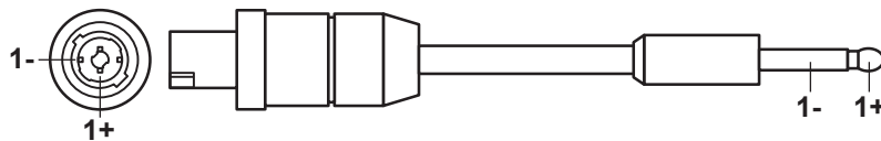
Speakon ® to 1/4" Wiring Diagram:
